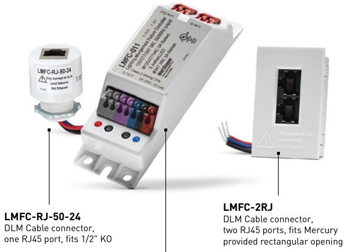
LMFC-011 0-10V dimming luminaire controller, mounts internally.
